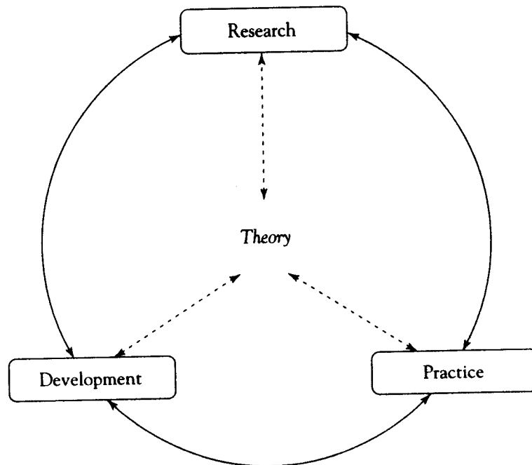
Theory-Research-Development-Practice Cycle
